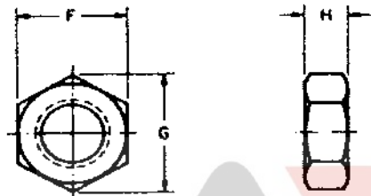
Hex Jam Nut, double-chamfered
