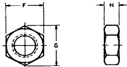
Heavy Hex Jam Nut, washer-faced and double-chamfered
